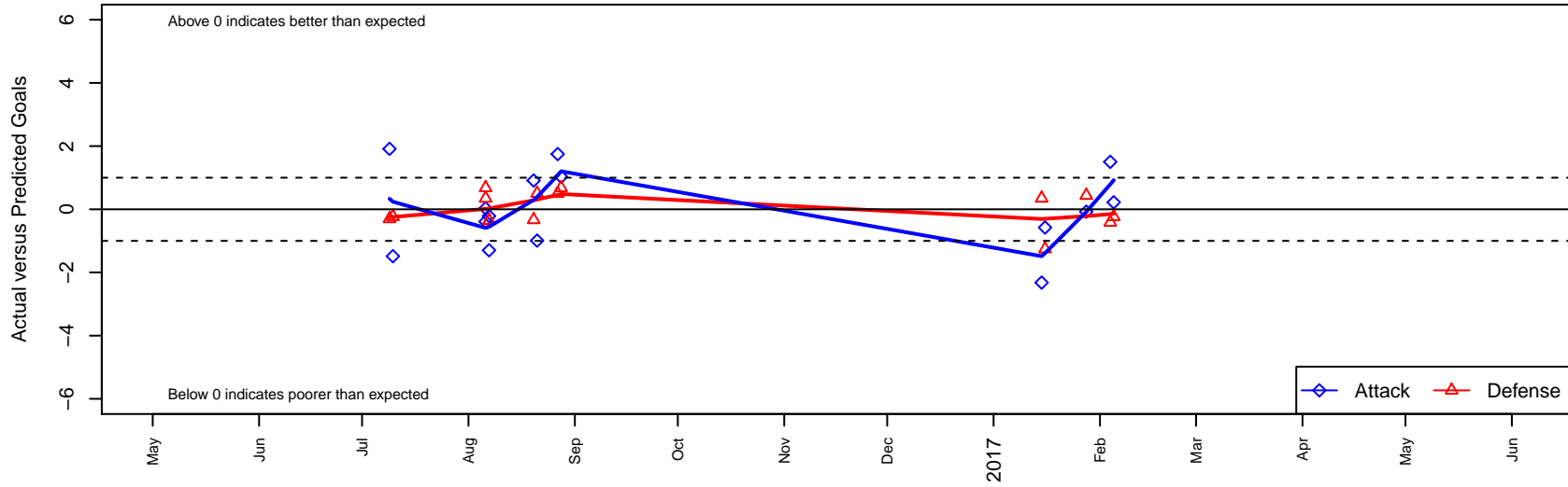
Oxnard United SC B03 Dots are actual minus expected GF (blue circles) and GA (red triangles). Blue line is smoothed change in attack strength. Red is smoothed change in defense strength.
